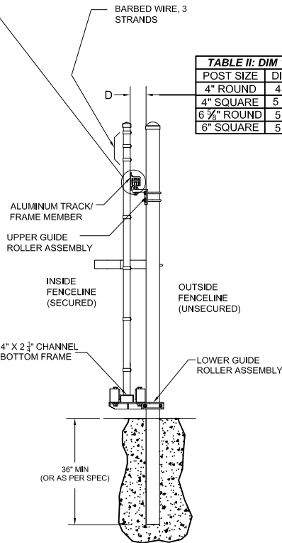
DETAIL VIEW A
