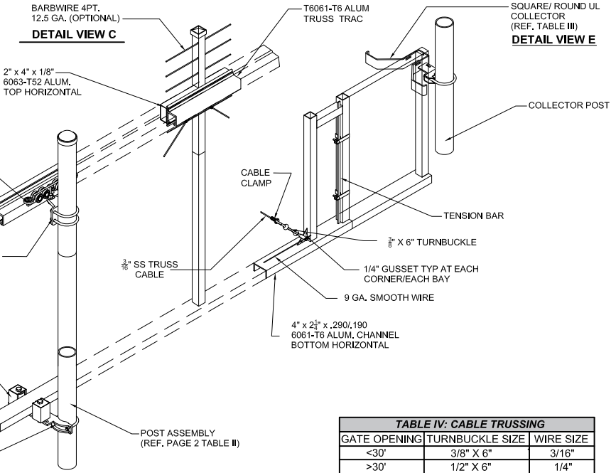
DETAIL VIEW B
